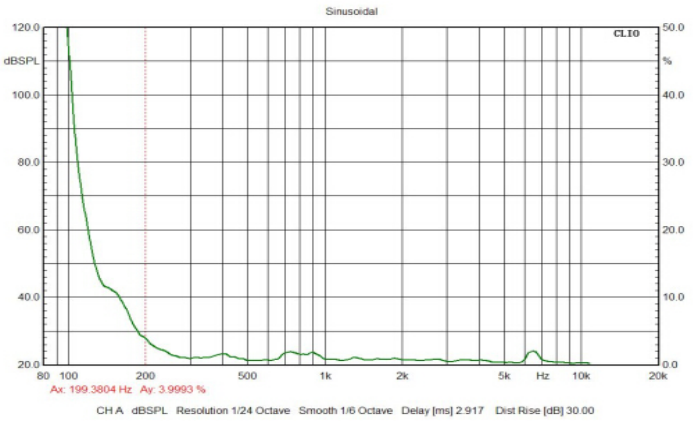
THD
