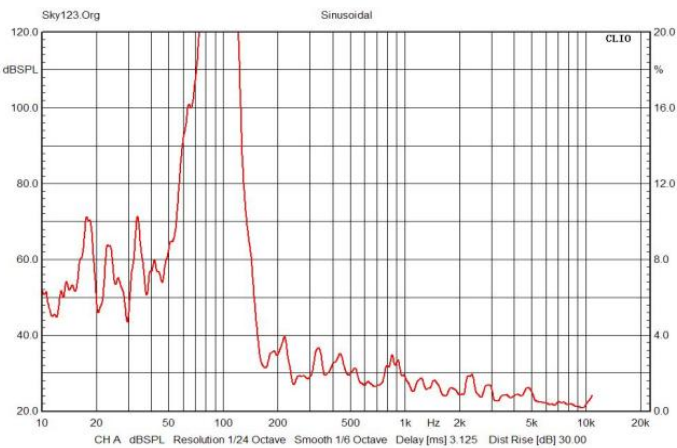
THD
