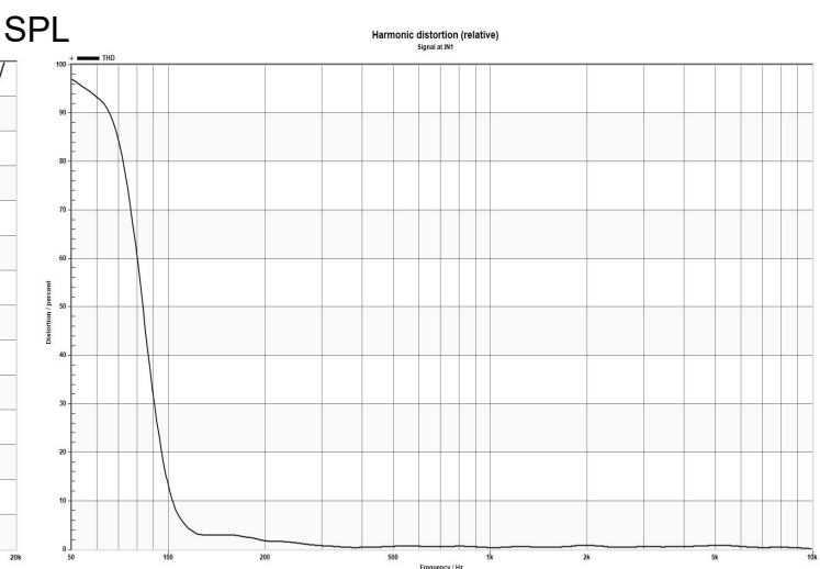
THD
