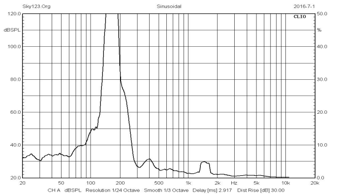
THD
