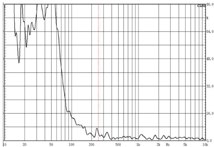
THD
