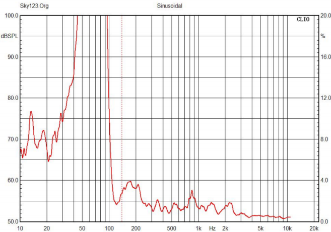
THD
